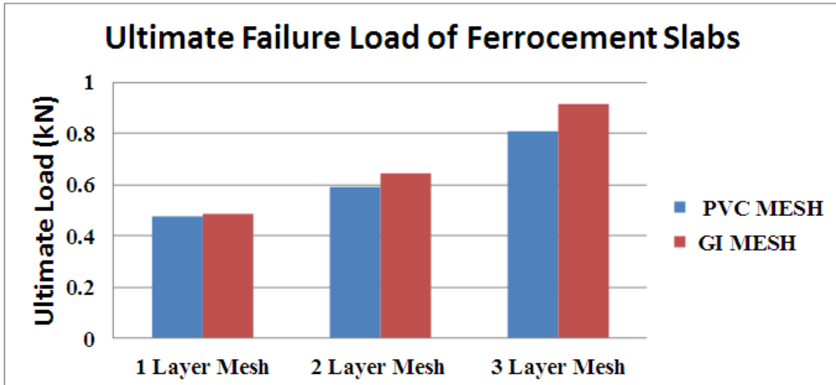
Fig. 4 Ultimate Flexural Load of Ferrocement Slabs (15mm thick)
