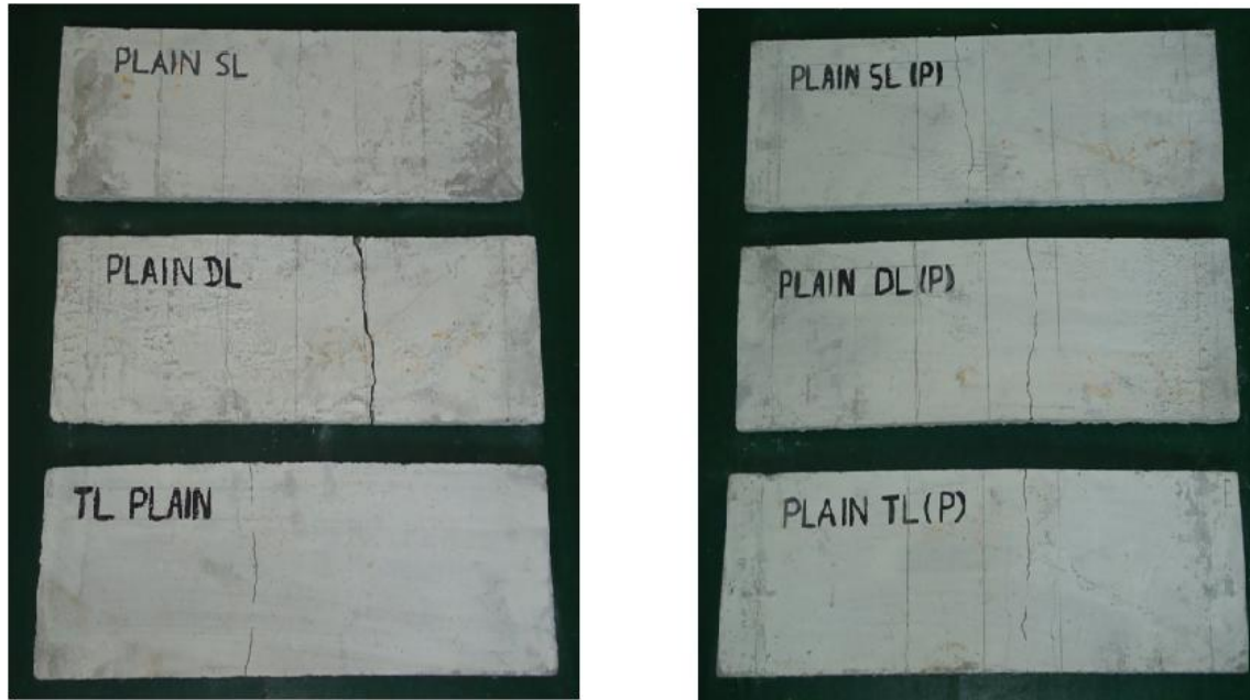
Fig. 8 Typical Crack-Pattern of Ferrocement Slabs cast with GI and PVC coated Weld Mesh, on ultimate failure loads
