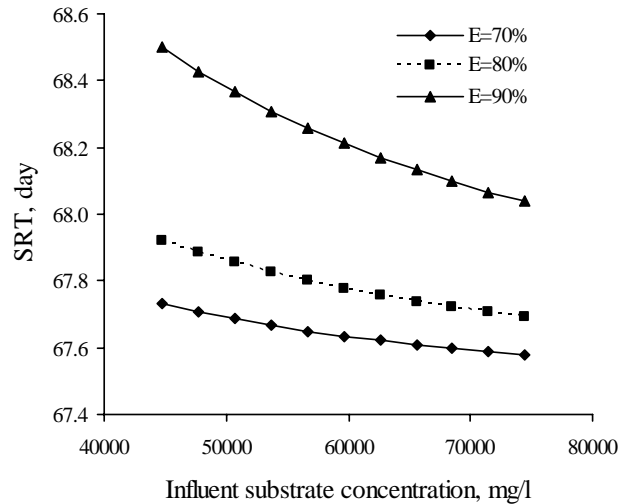
Fig. 4 Variation of SRT of anaerobic reactor for MSW digestion with influent concentration
