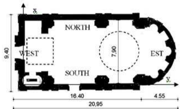
Fig. 10 Horizontal section
