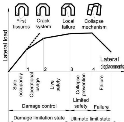
Fig. 1 Behaviour of a masonry triumphal arch
