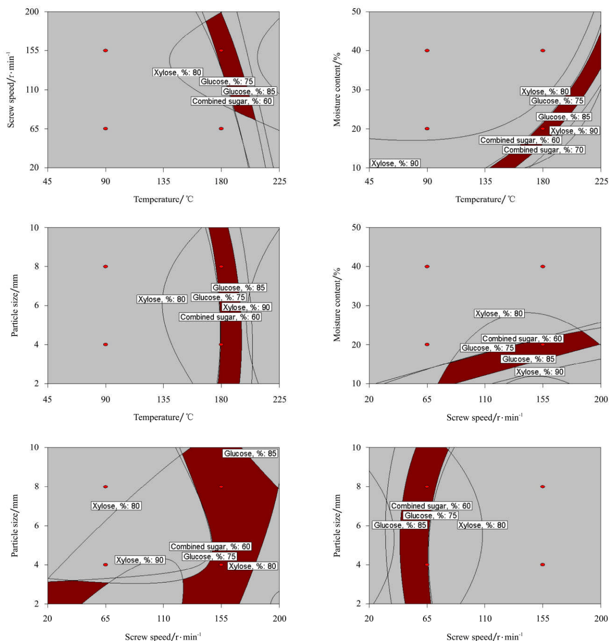
Figure 4 Superimposed contours for sugar recovery responses as affected by temperature, screw speed, moisture content, and particle size
