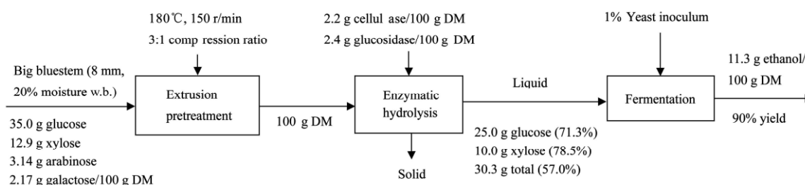
Figure 6 Mass balance diagram extrusion pretreatment followed by fermentation
