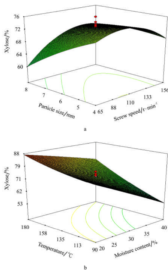
Figure 2 Effects of independent variables interaction on xylose recovery (when other factors fixed at the center point)
