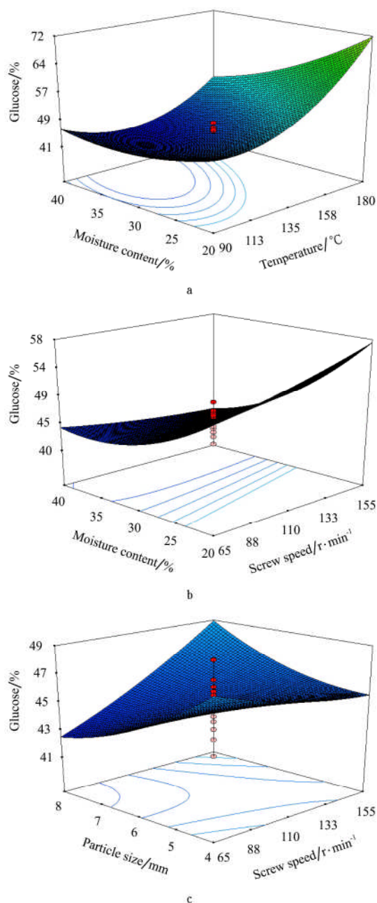
Figure 1 Effects of independent variables interaction on glucose recovery (when other factors fixed at the center point)
