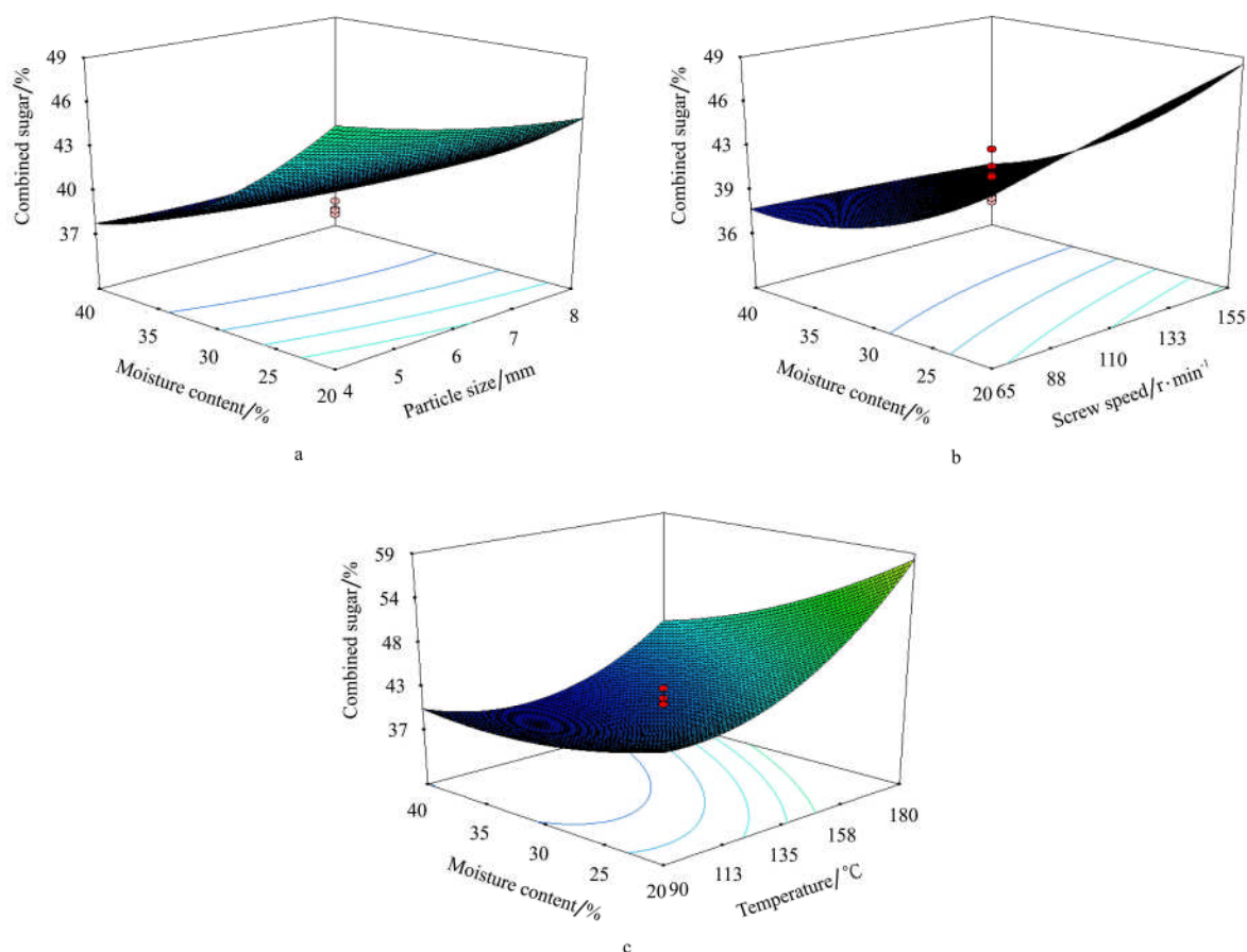
Figure 3 Effects of independent variables interaction on combined sugar recovery (when other factors fixed at the center point)
