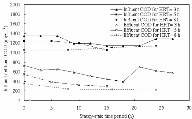
Fig. 2 Influent and effluent COD profile during continuous study
