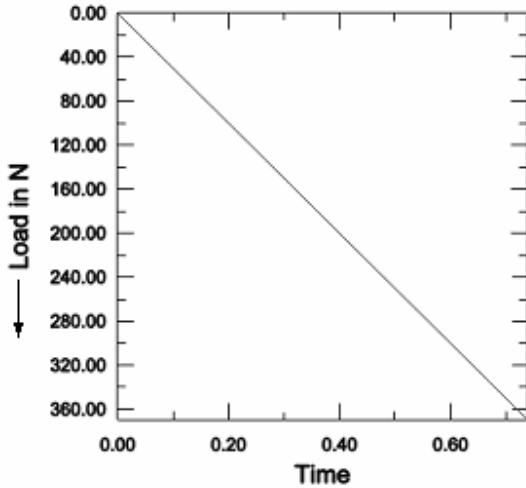
Fig. 7 FE predicted load Vs. time plot for H11 steel specimen
