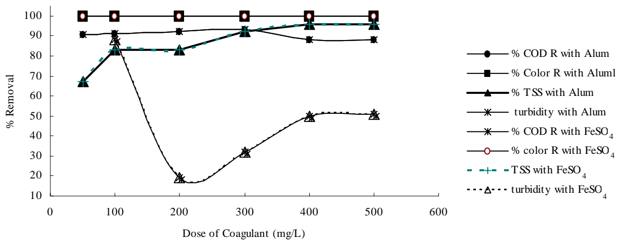
Fig. 3. % Removal of Color, COD & TSS and turbidity for different doses of coagulant (At optimum pH=8.2 for Alum Or at pH=9.4 for \text{FeSO}_4 )
