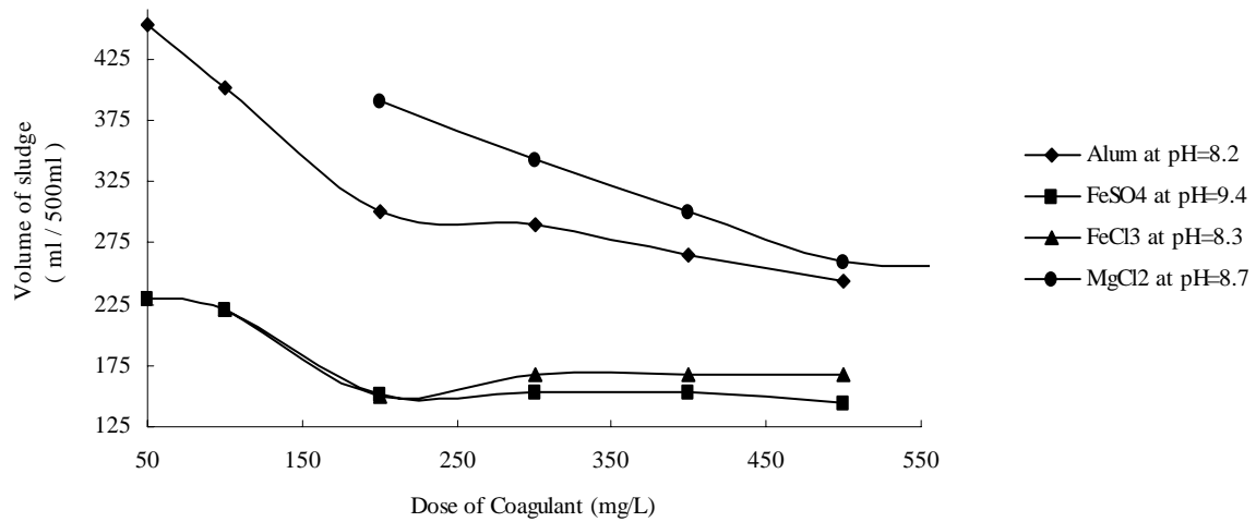
Fig. 4. Settled sludge volume for different coagulants at their optimum pH
