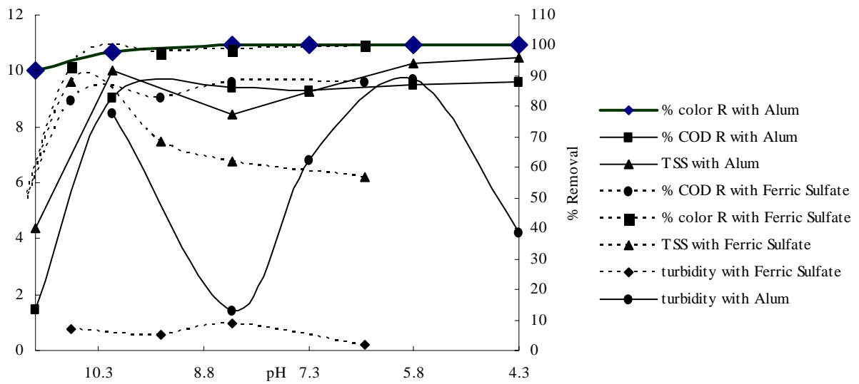
Fig.1. % Removal of Color, COD & TSS and turbidity for different pH. (For 400 mg/L Alum or 400 mg/L of \text{FeSO}_4 )
