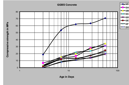
Figure 5 compressive strength of GGBS concrete
