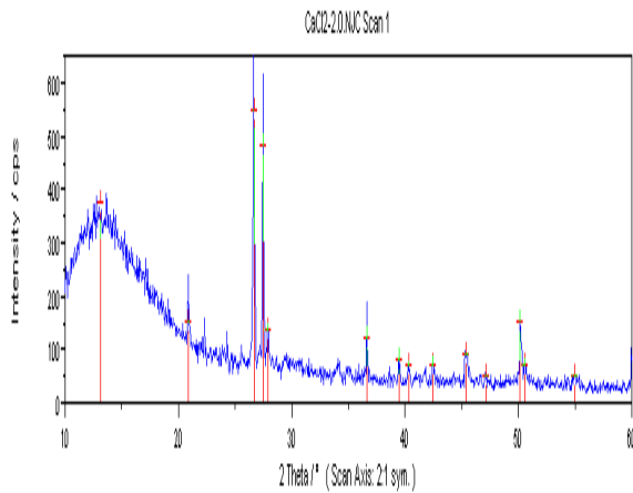
Fig.10. Powder X- Ray Diffraction Pattern for the Admixture Cement (PPC Cement + 10% Silica Fume) Mortar Cubes Prepared With CaCl 2 (0.5 G/L and 2.0 G/L) in Deionised Water The comparison of this powder X- ray diffraction pattern with that of the control mix indicates that the formation of tricalcium silicate (3CaO. SiO 2 ). This is characterized by the presence of d-spacing's 6.461 Å, 3.342 Å and 2.281 Å, these peaks not being present in the pattern for the control mix. The possible chemical reaction upon the hydration of cement with mixing water containing CaCl 2 is as follows:
