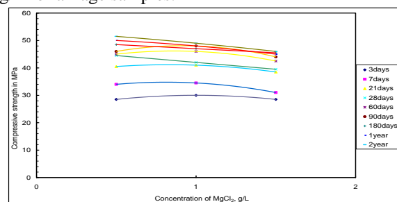
Fig.6. Variation of Compressive Strength of Admixture Cement (PPC Cement + 10% Silica Fume) Mortar Cubes at Different Ages Corresponding To Various Concentrations of Mgcl 2 in Deionised Water
