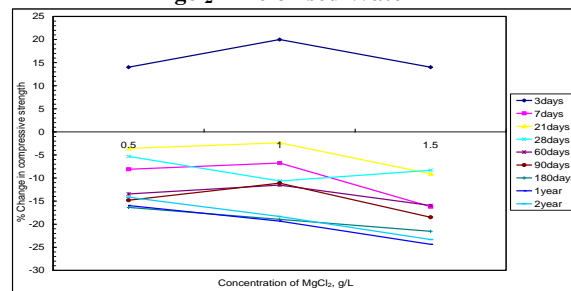
Fig.7. Percentage Variation Of Compressive Strength Of Admixture Cement (PPC Cement + 10% Silica Fume) Mortar Cubes At Different Ages Corresponding To Various Concentrations Of Mgcl 2 In Deionised Water
