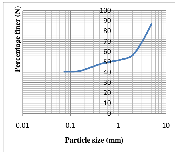
Figure 1.1: Particle size distribution curve Ch6+950
