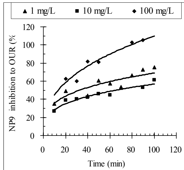
Fig. 4 Inhibition to OUR for different concentrations of Trigetol NP-9 during a 2h OUR test using activated sludge samples collected July 2007
