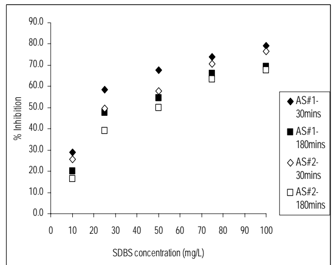
Fig. 7 Inhibition to OUR in the presence of SDBS
