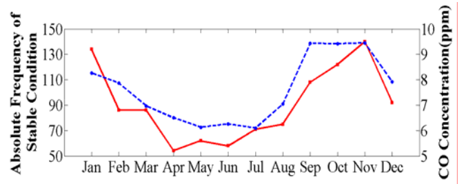
Fig. 7 Time series of absolute frequency of stable conditions and CO concentration for 2000-2005 (Solid line: Stability; Dashed line: CO average concentration)
