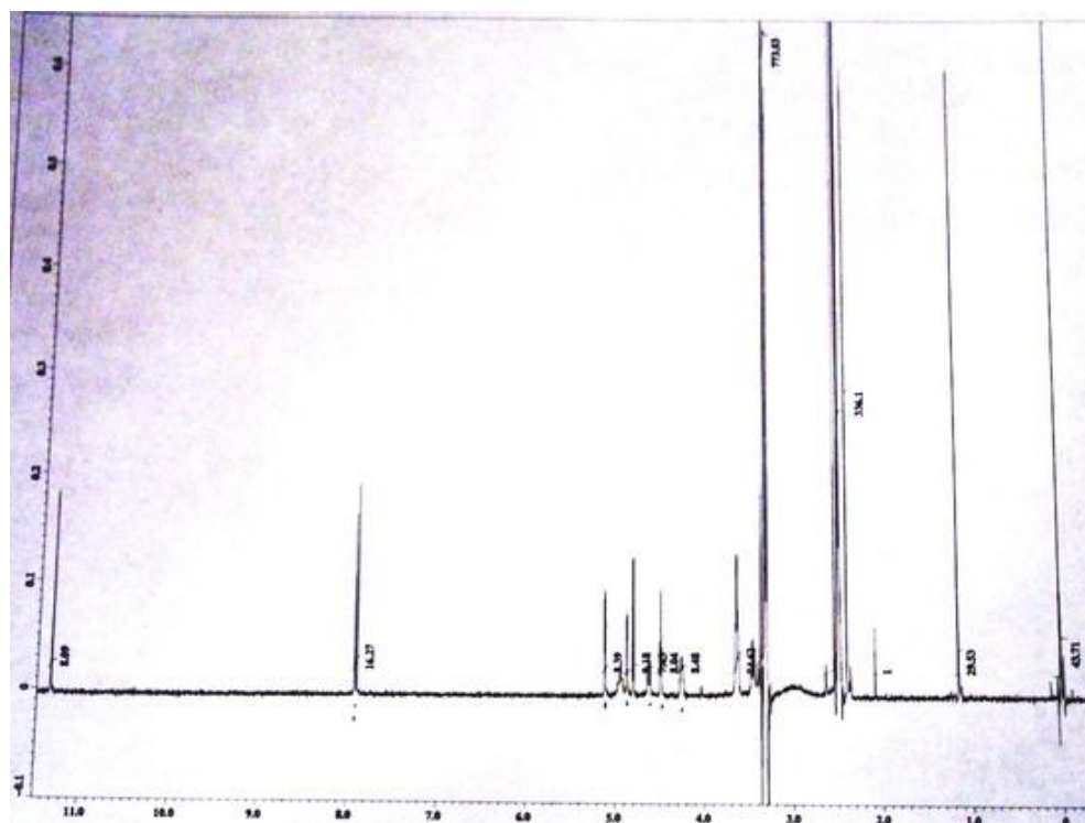
Free Induction Decay(X-axis: Time|Y-axis: Amplitude) NMR Spectrum(X-axis: Chemical Shift (ppm)|Y-axis: Amplitude)
