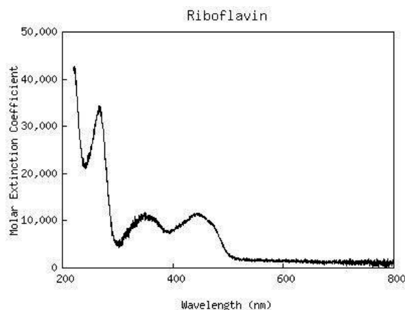
Frequency Resolved Visible Absorption Spectrum
