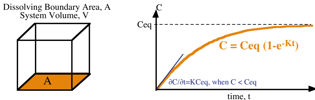
Figure 2. Evolution of concentration with boundary source.
