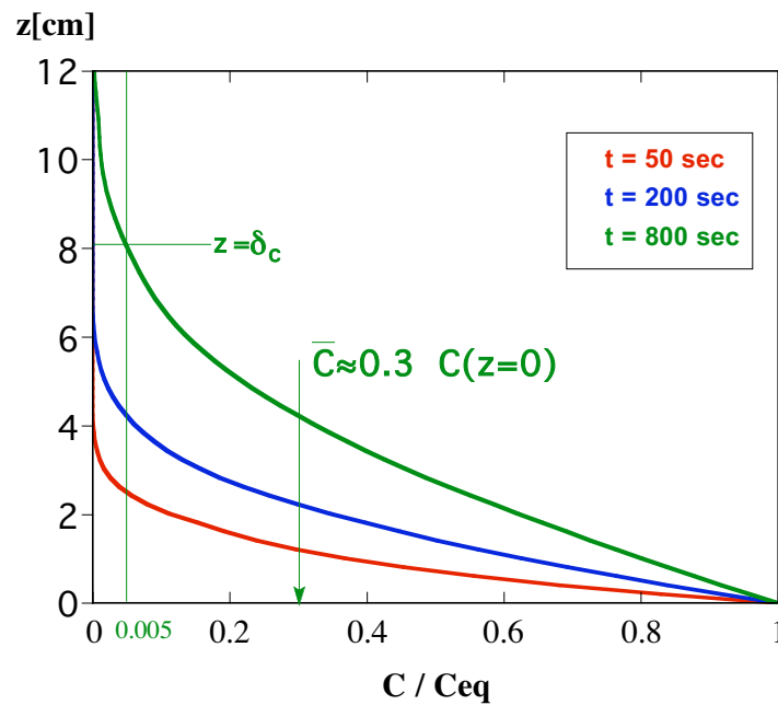
Figure 3. Development of concentration boundary layer above constant concentration boundary. The concentration at the boundary is in equilibrium with the solid phase, C(z=0) = C_{eq} .
