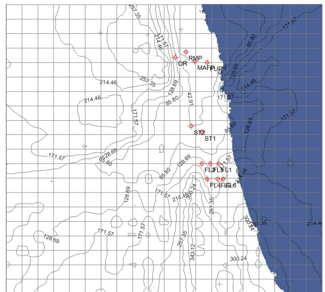
Fig. 5 Contour map of SO 2 concentration
