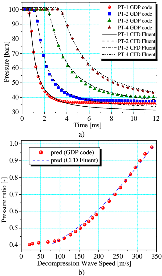
Fig. 5 Predicted pressure time history at different PT locations (a) and decomposition wave speed as a function of pressure ratio (b)
