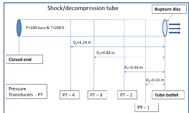
Fig. 4 Schematic of the decompression tube
