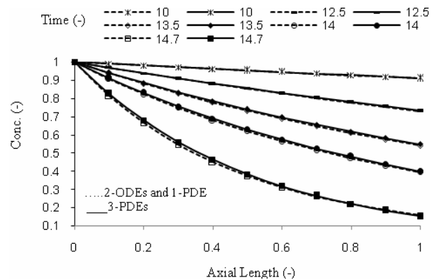
Fig. 2 Propylene concentration variation along the axial length
