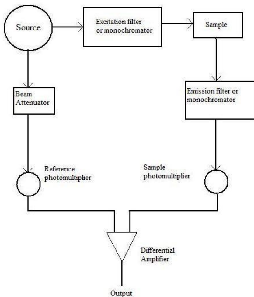
Figure 2. Schematic of Fluorescence Spectrometer
