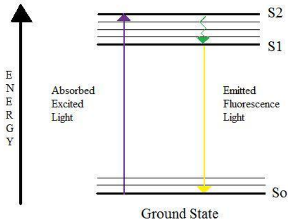
Figure 1. Jablonski diagram
