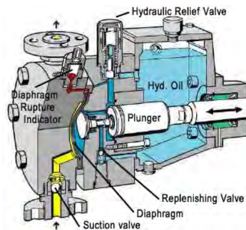
Figure 1.6B Double diaphragm pumps (Lewa Pumps)
