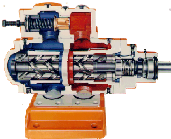
Figure 1.14 Three-spindle screw pump – Alweiller pumps
