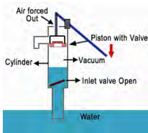
Figure 1.4 Reciprocating hand pump in suction stroke
