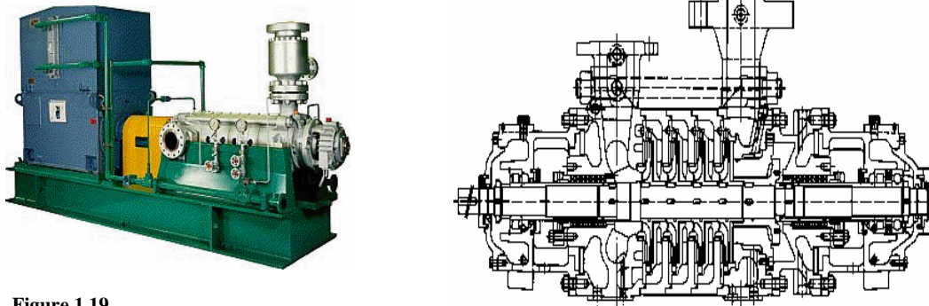
Figure 1.19 Multistage pump
