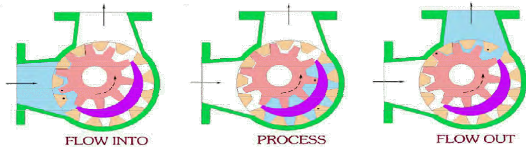
Figure 1.8 Internal gear pump
