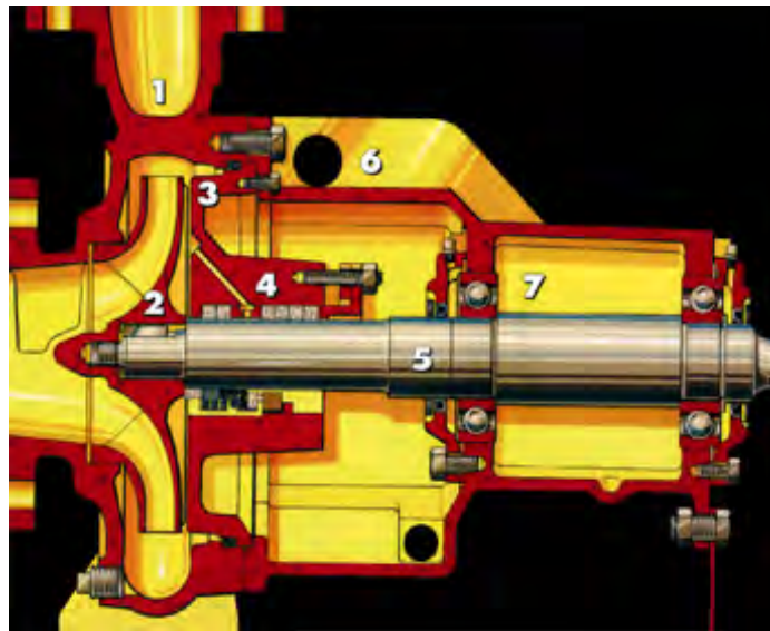
Figure 1.17 Centrifugal pump – basic construction
