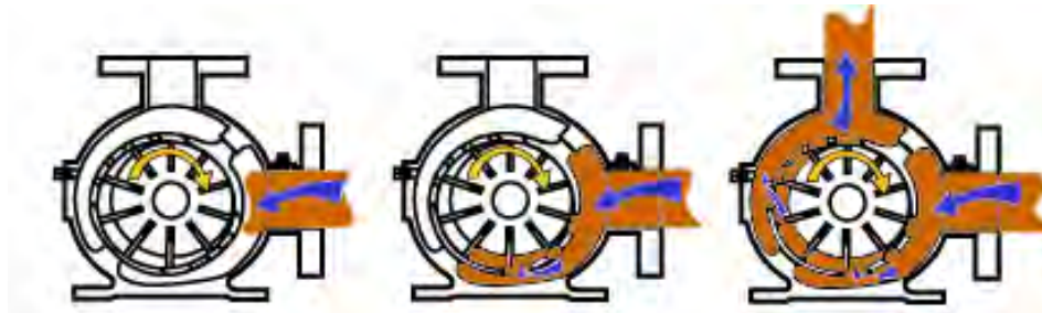
Figure 1.10 Vane pump
